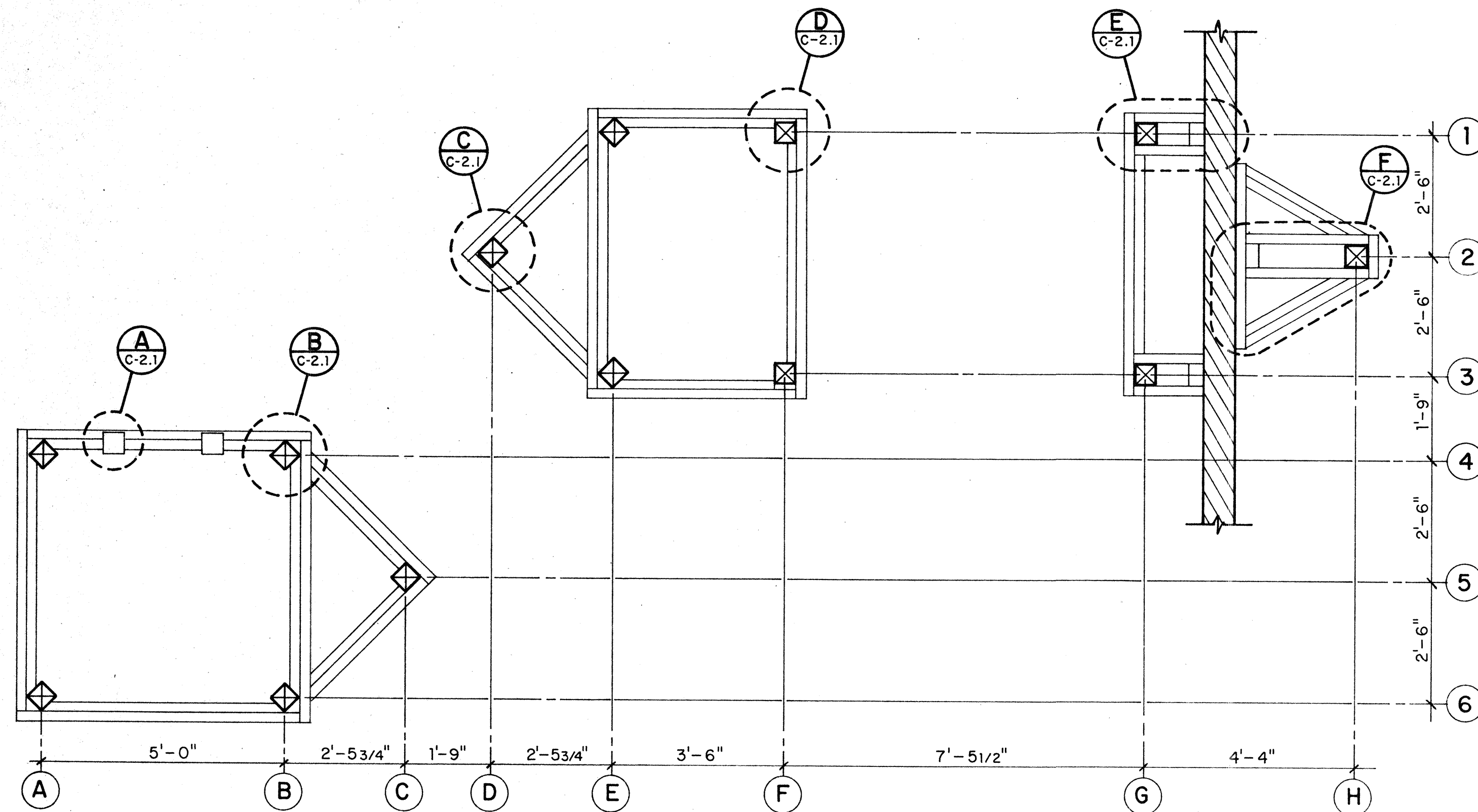
STRUCTURE "C" FOUNDATION PLAN
