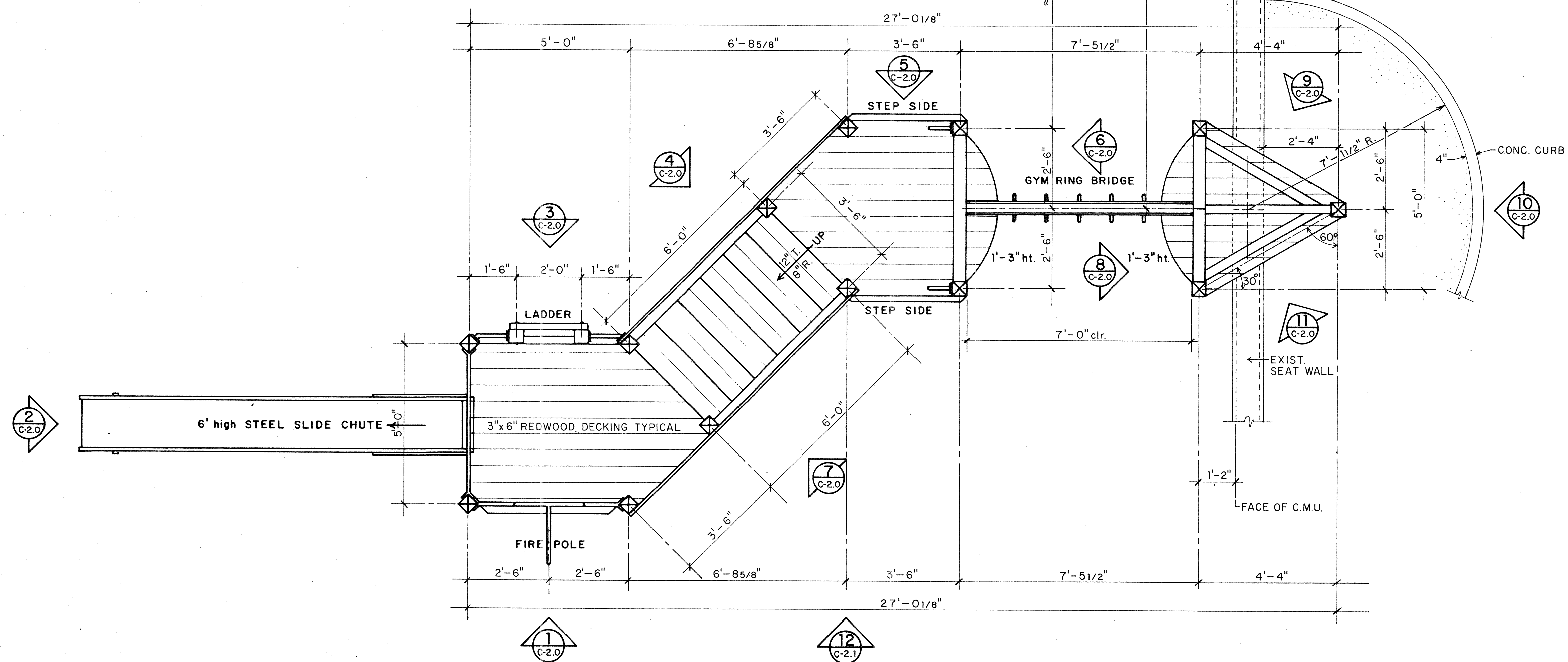
CLIMBING STRUCTURE "C" PLAN
